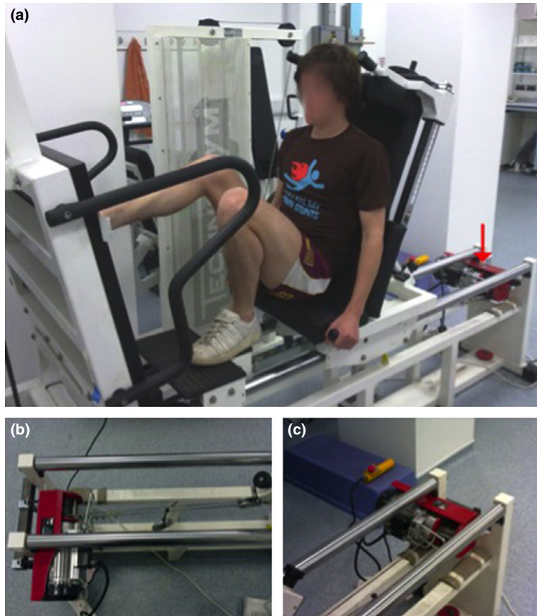
Figure 1 Subject on the Technogym leg press modified ad hoc with the special electric engine visible on the right corner indicated by the arrow (a). The electric winch attached to the chair via steel cable; (b) shows how the winch was connected to the chair (the red arrow indicates a counterweight that prevented the cable from becoming too slack and getting damaged); (c) presents the site where the engine was placed.
